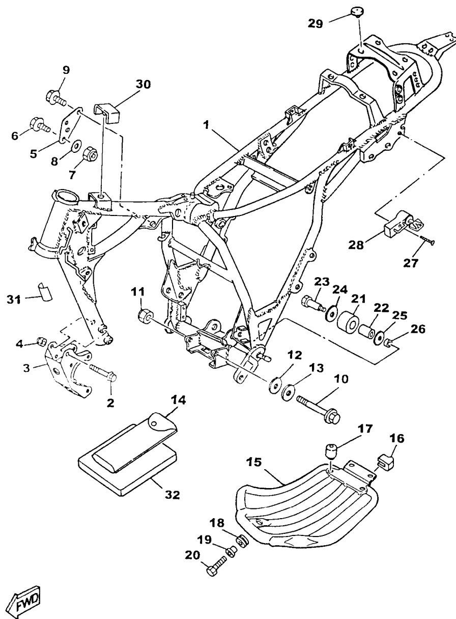
FIG. 17 - CHASSIS
